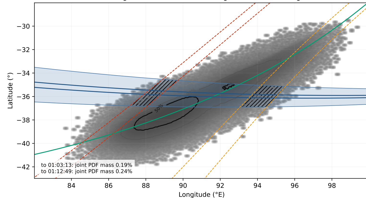
H01W Table 1: 00:49:58 UTC, bearing 260.41° blue: bearing band; dashed: H08S range-difference timing bands
