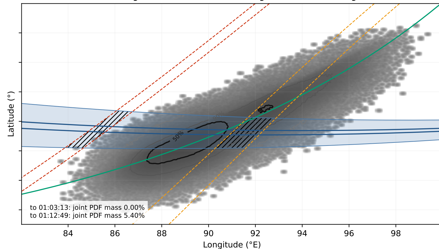
H01W Table 1: 00:53:31 UTC, bearing 257.58° blue: bearing band; dashed: H08S range-difference timing bands
